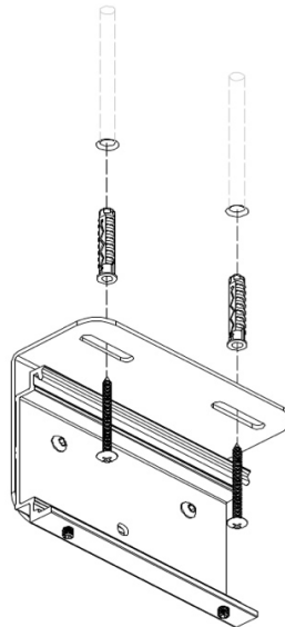
Fig. 1B – Ceiling Mounting
