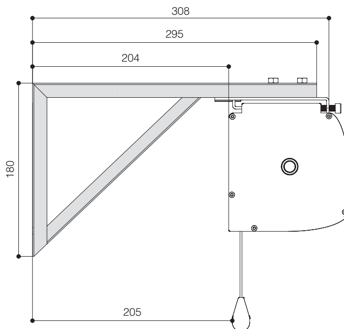
Short wall extension bracket L = 295
