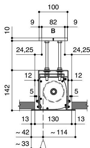
HOLE IN FALSE CEILING AND FIXING POINTS INTO CEILING
