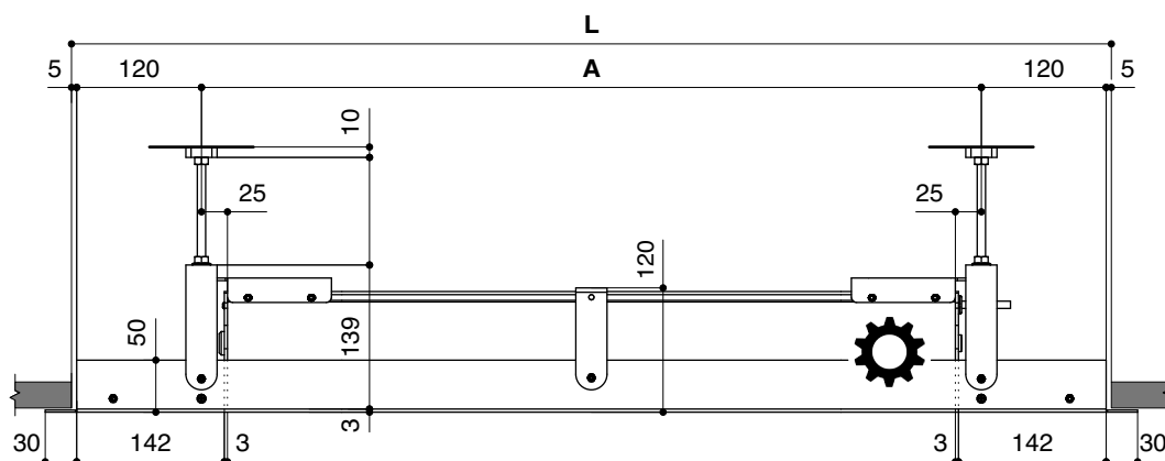
FRONT VIEW TRIM KIT COMPACT
