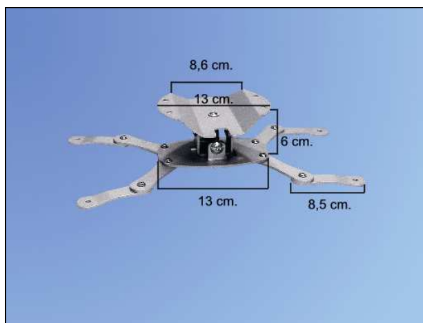
PROJECTOR ARM B-7 – misure principali
